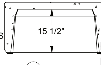
5 SECTION
