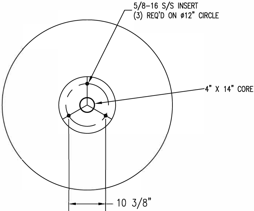
3 BOTTOM VIEW
